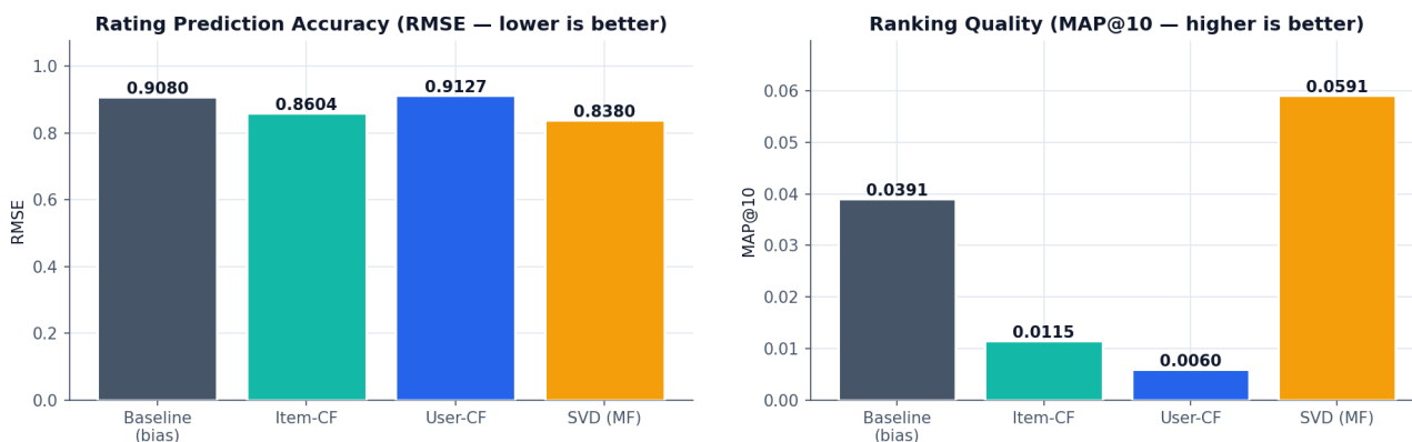
Figure 2. Mandatory metrics. Left: RMSE (lower better) — SVD best at 0.838. Right: MAP@10 (higher better) — SVD best at 0.059, \sim 1.5\times the baseline.
