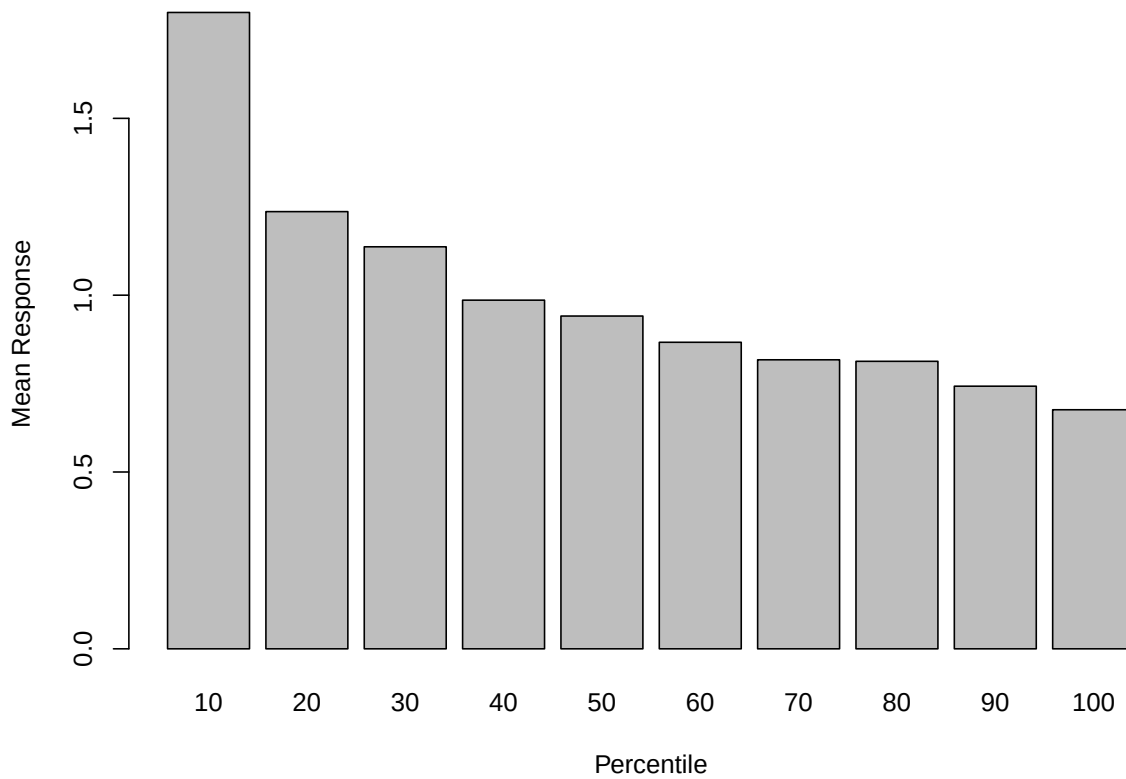
Decile-wise lift chart
