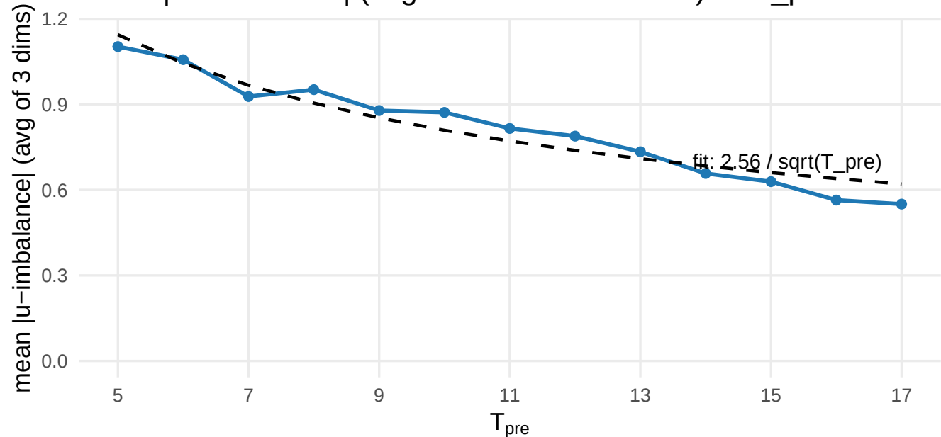
Mean |u-imbalance| (avg across 3 factor dims) vs T_pre
