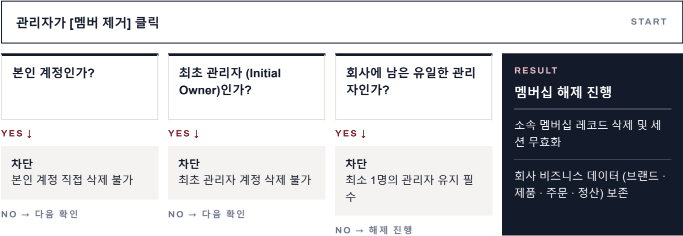
DIAGRAM 05 · MEMBER REMOVAL DECISION FLOW
