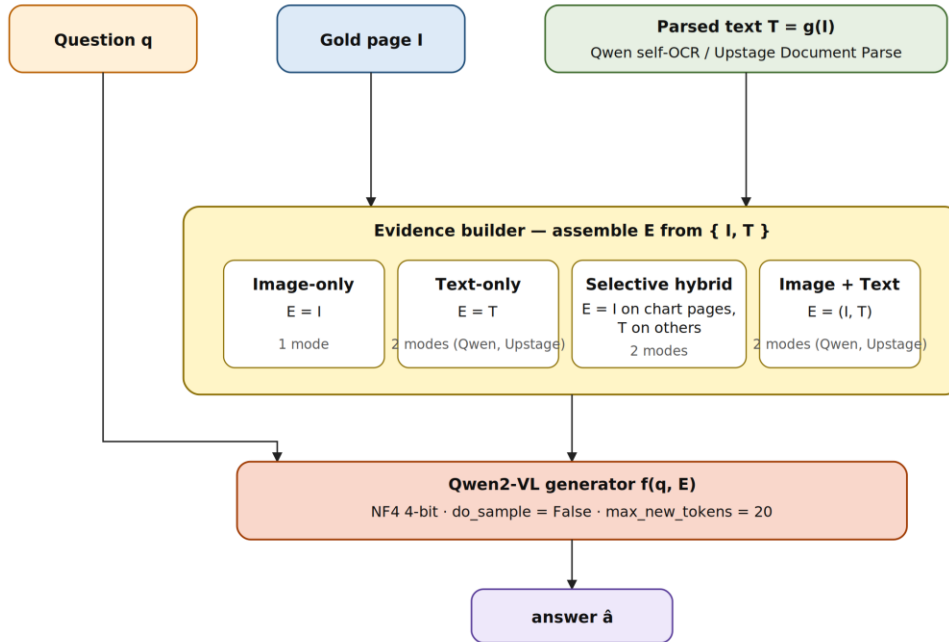
225 Figure 1. Oracle-controlled evidence pipeline. Question q is paired with the gold page I (oracle qrels, top-1) and the parsed text T = g(I) , where g is either Qwen self-OCR or Upstage Document Parse. The evidence builder assembles the evidence set E according to the selected mode; the Qwen2-VL generator decodes the answer from (q, E) under NF4 4-bit quantisation with do\_sample=False and max\_new\_tokens=20 . Only the contents of E vary across the seven modes.
