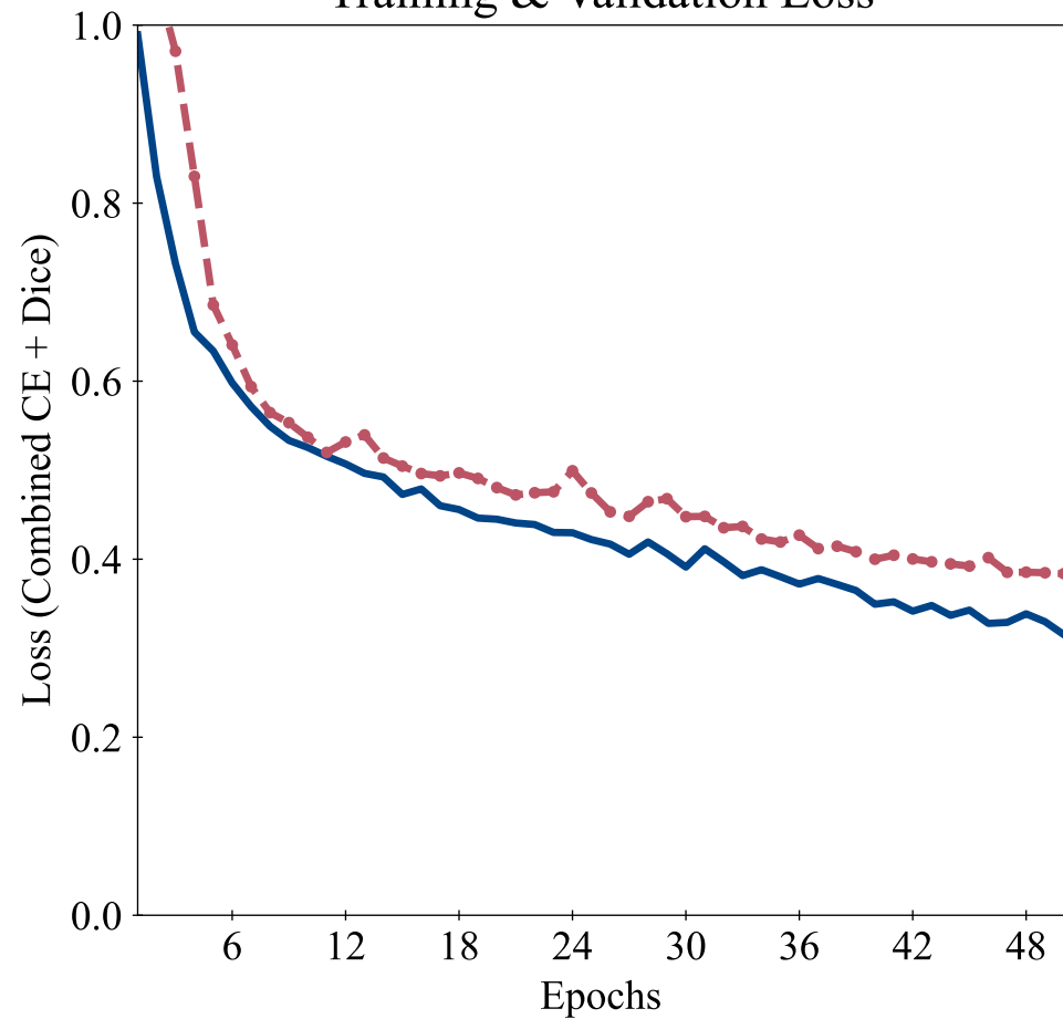
Training & Validation Loss
