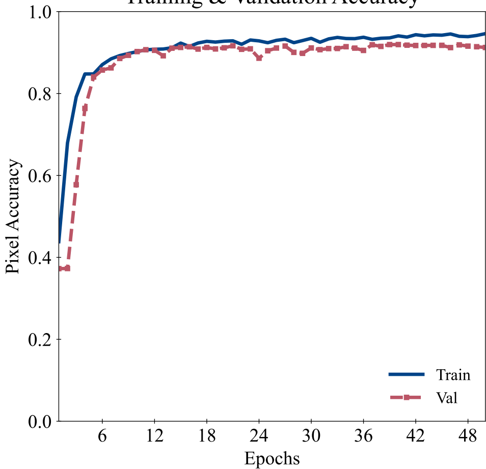
Training & Validation Accuracy
