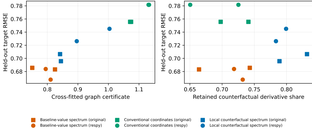
FIGURE 3. Generator certificate, derivative share, and held-out target risk
