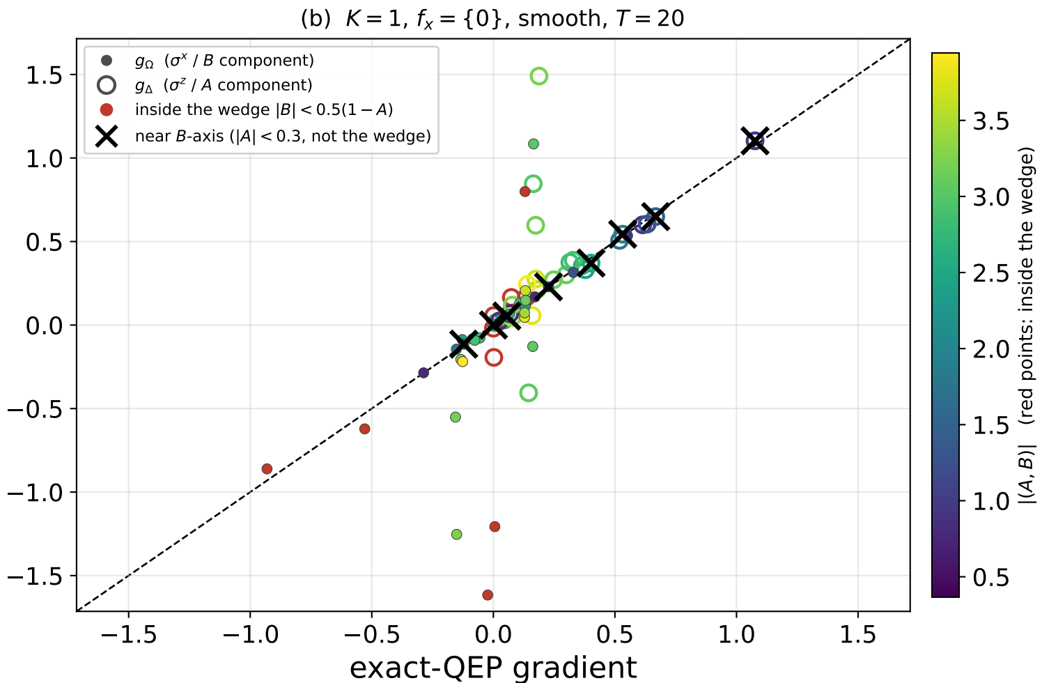
Two different outlier populations: Landau-Zener (red) vs \sigma^x -saturation near the B -axis (black \times )
