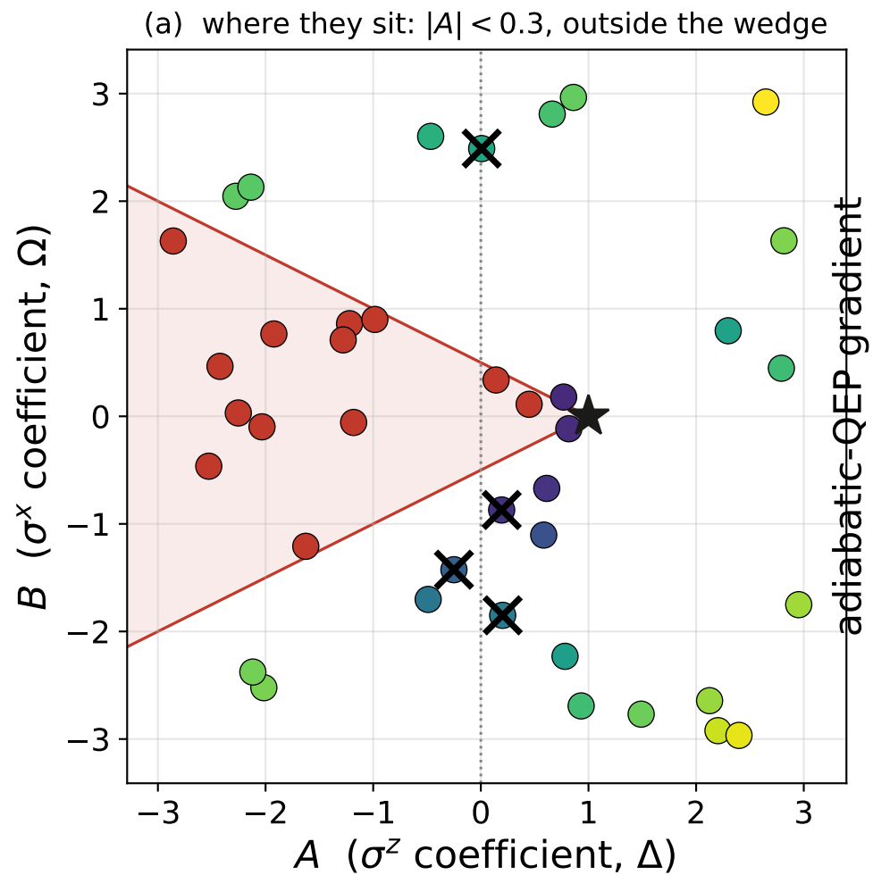
Two different outlier populations: Landau-Zener (red) vs \sigma^x -saturation near the B -axis (black \times )
