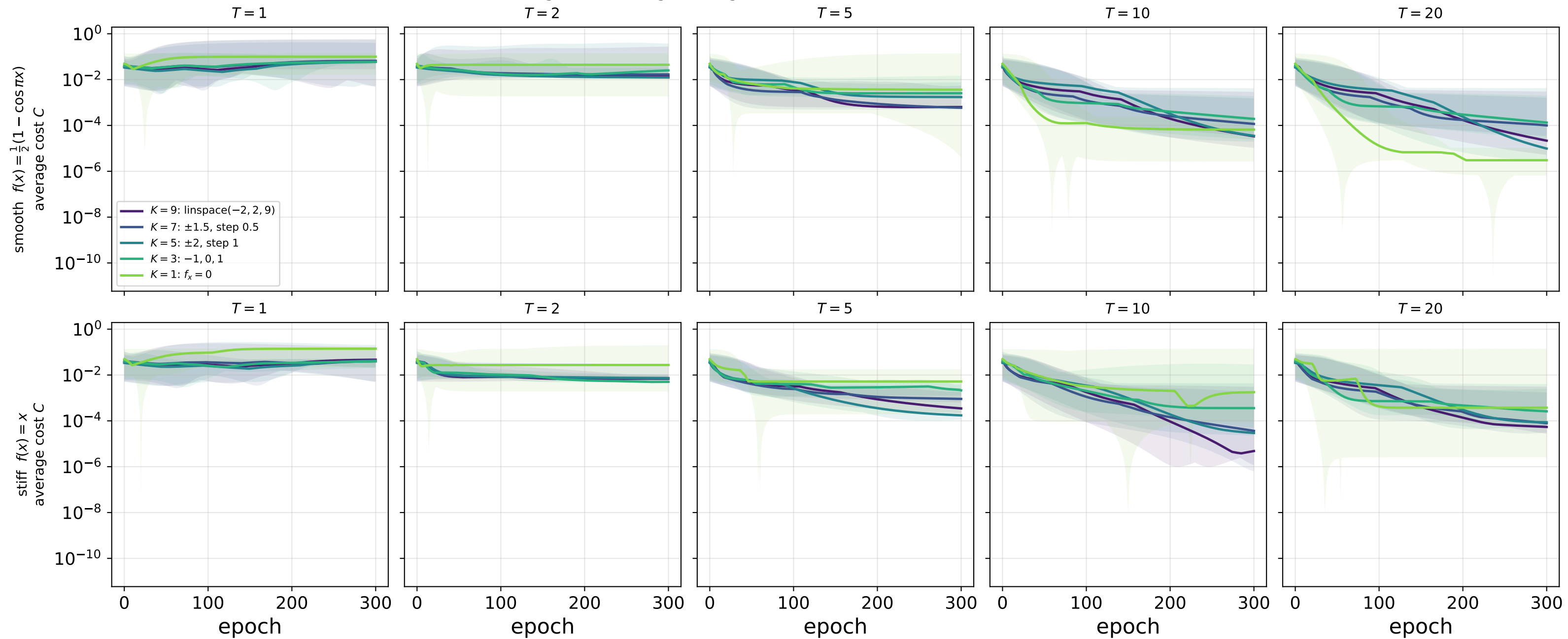
Average cost during training, median over 6 inits (band = min-max)
