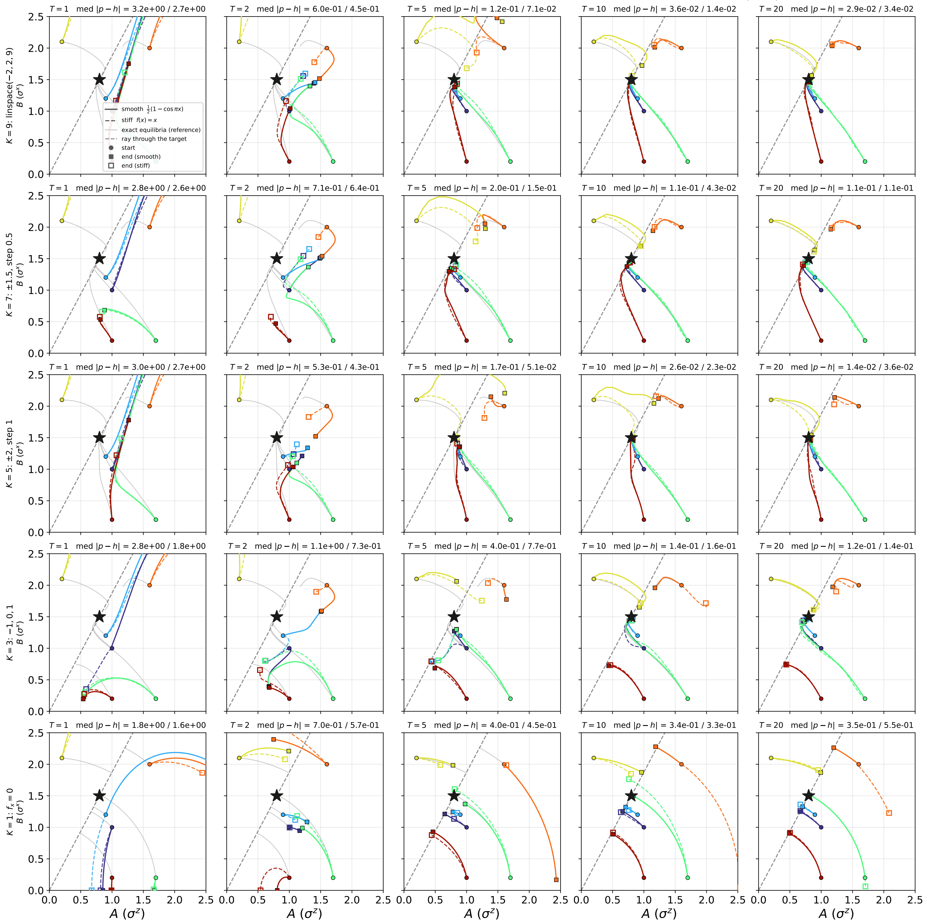
Training with fewer probe fields — both schedules (solid = smooth, dashed = stiff, colour = initial point); panel titles: median final |p - h| smooth / stiff
