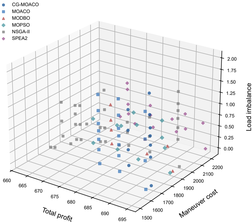
Pareto front: area_s5_t100
