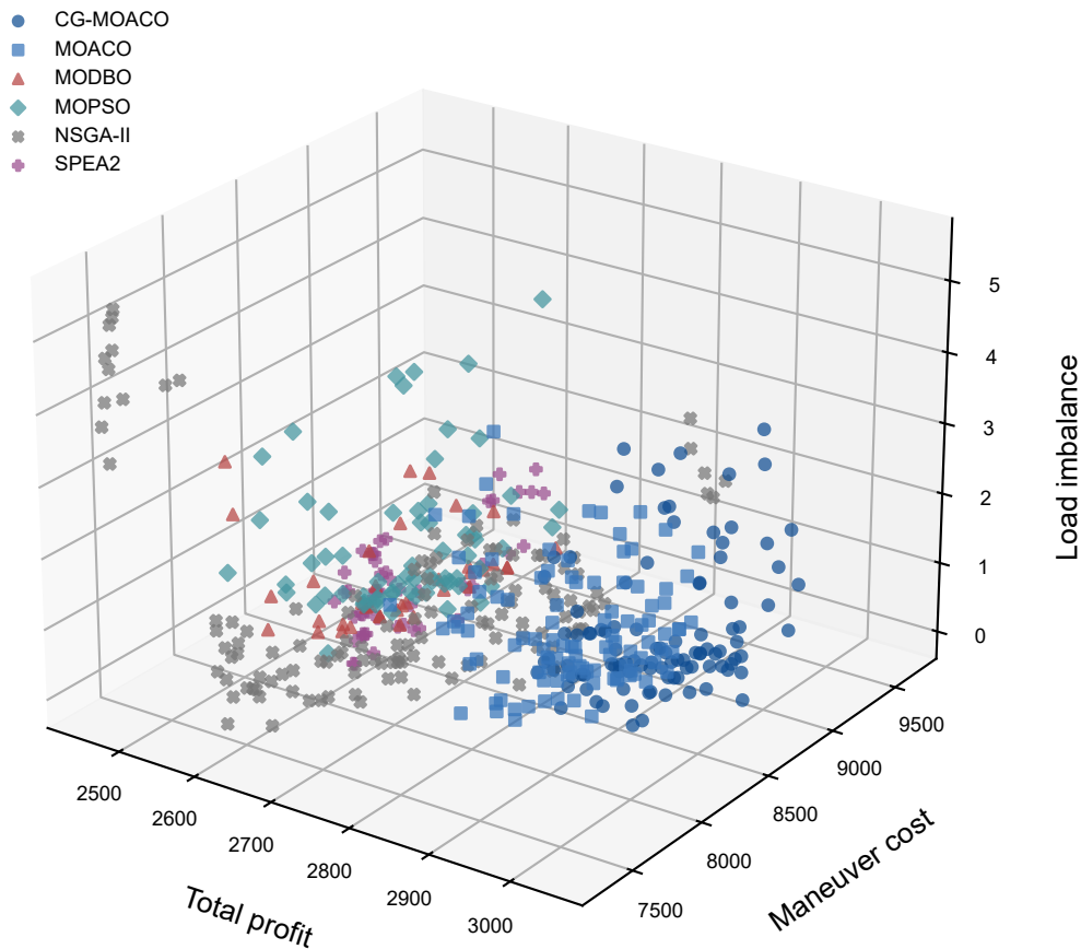
Pareto front: area_s5_t500
