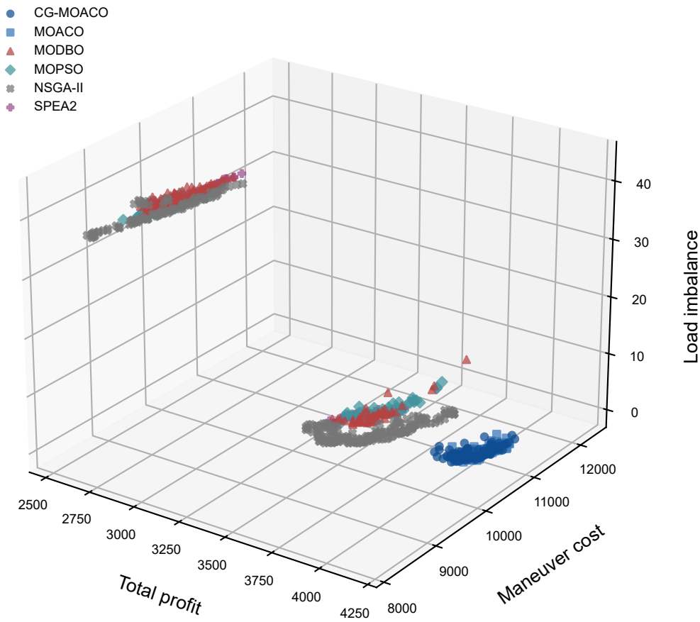
Pareto front: area_s5_t900
