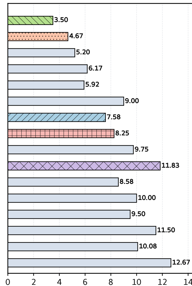
Qwen 27B
