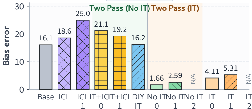
BBQ Disambig.
