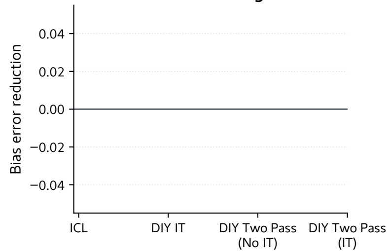
BBQ Disambig.
