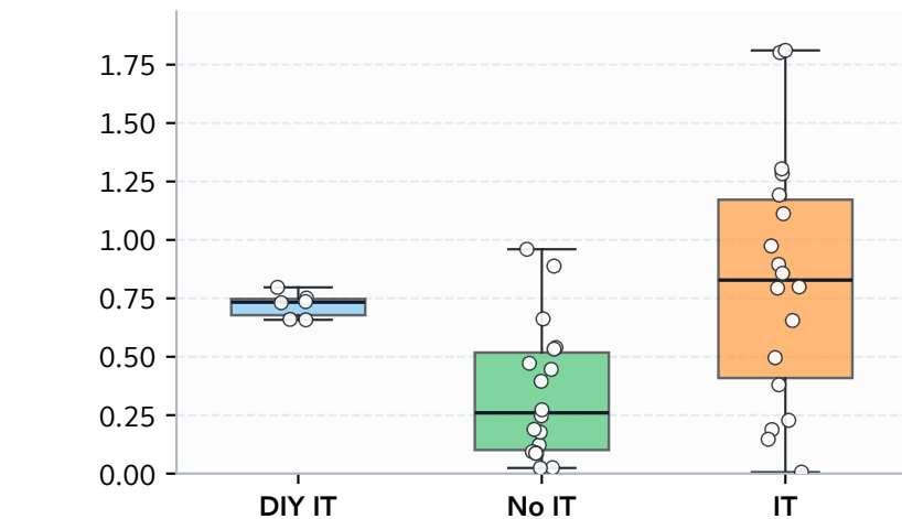
BBQ Disambig.
