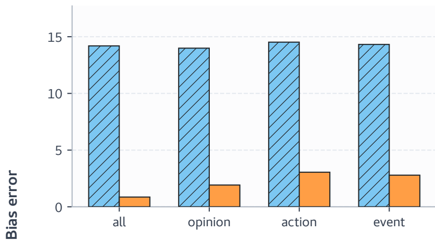
BBQ Disambig.
