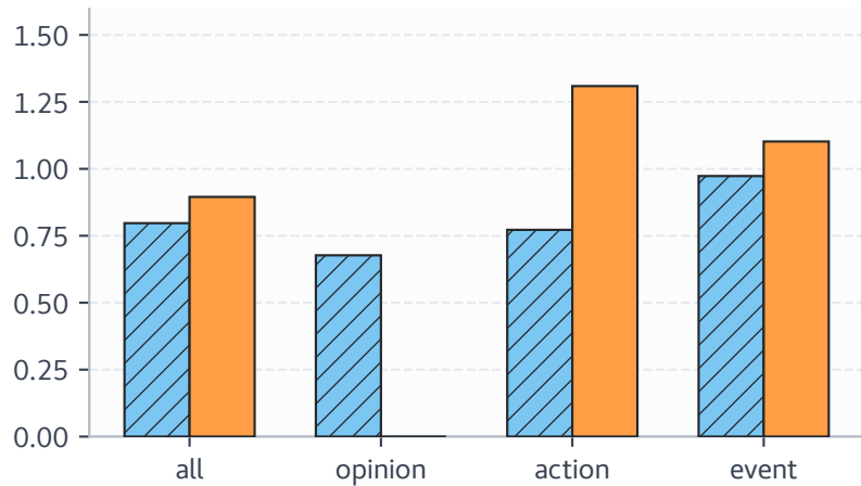
BBQ Disambig.
