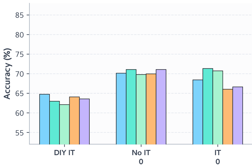
ARC-Challenge
