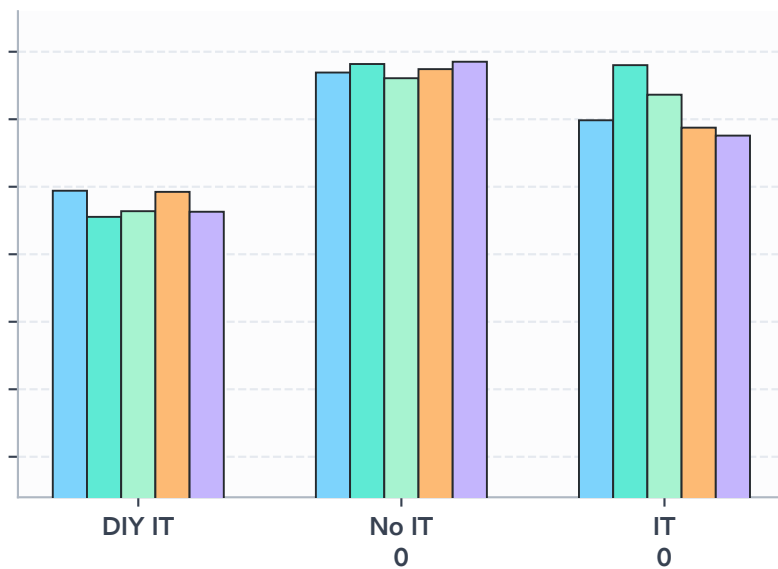
ARC-Easy
