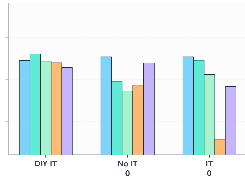
Balanced COPA
