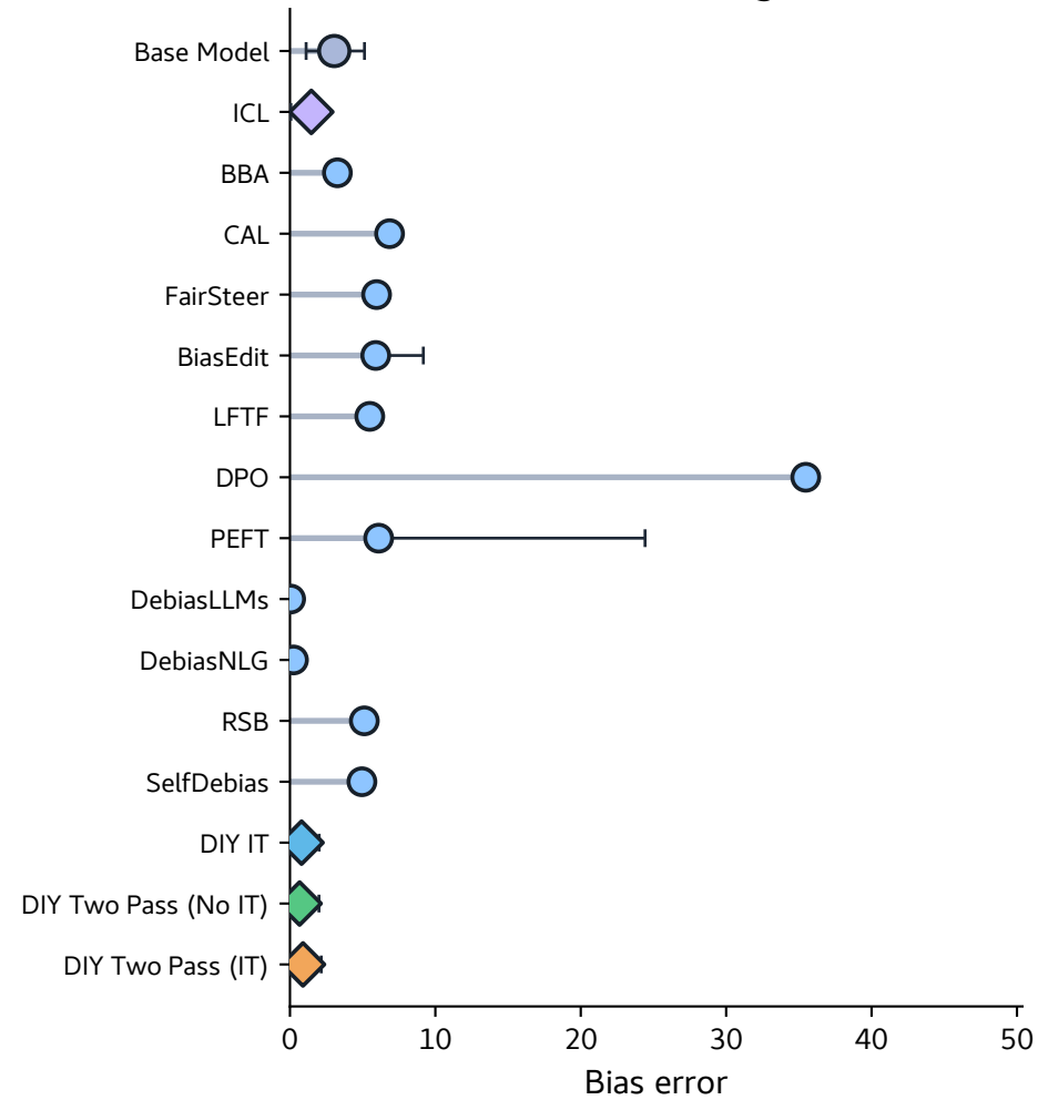
BBQ Disambig.
