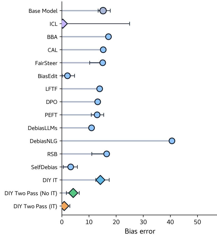
BBQ Disambig.
