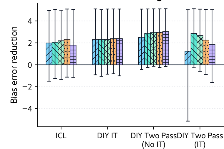
BBQ Disambig.
