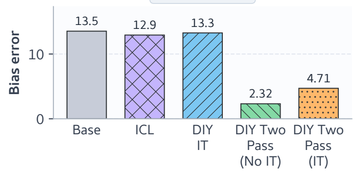
BBQ Disambig.
