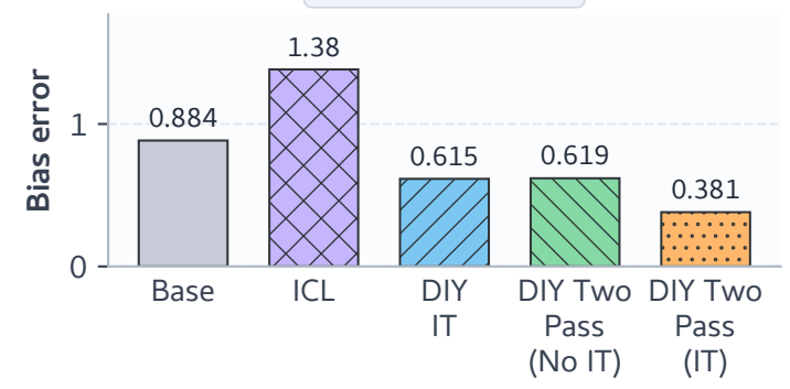
BBQ Disambig.
