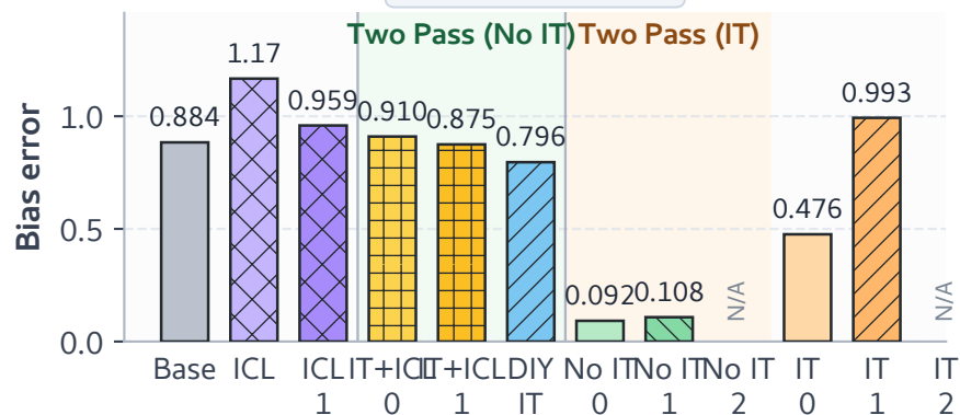
BBQ Disambig.
