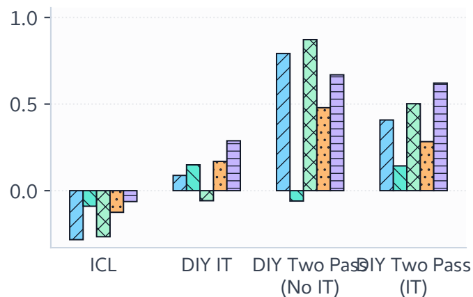
BBQ Disambig.
