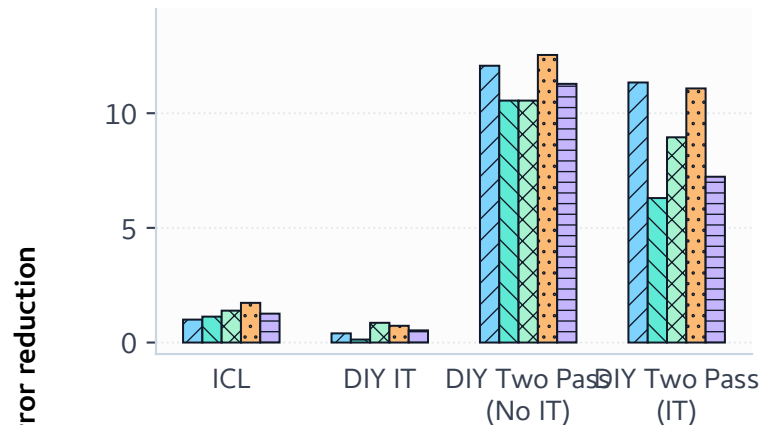
BBQ Disambig.
