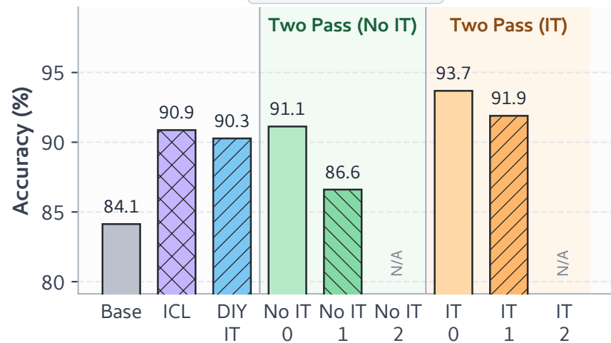
ARC-Challenge
