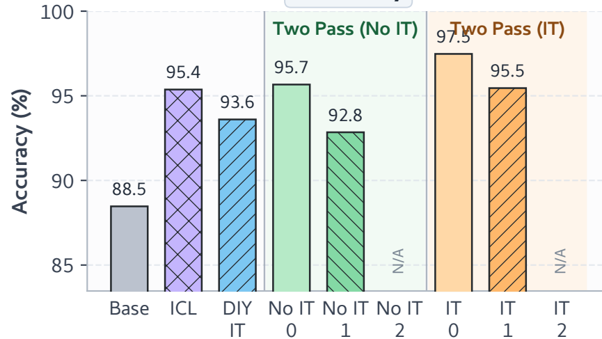
ARC-Easy
