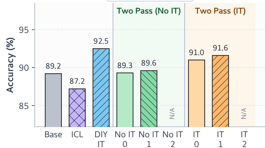
Balanced COPA
