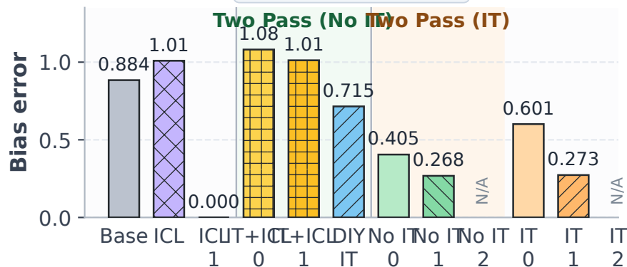
BBQ Disambig.
