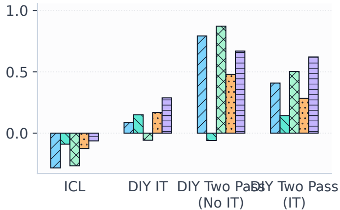
BBQ Disambig.
