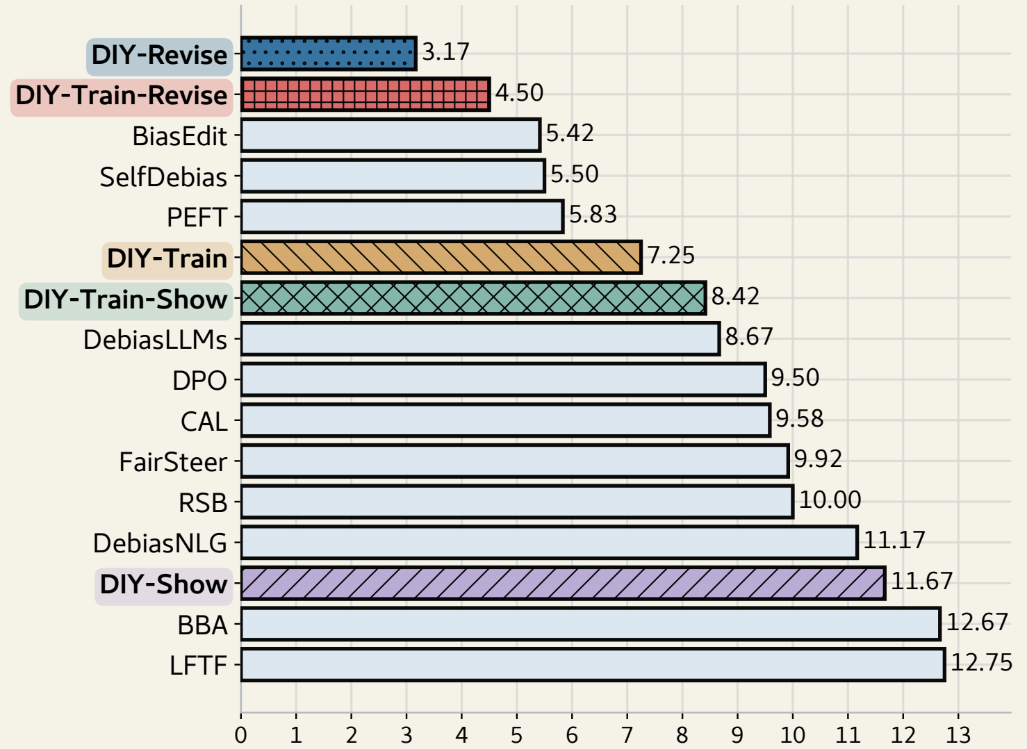
Qwen 27B
