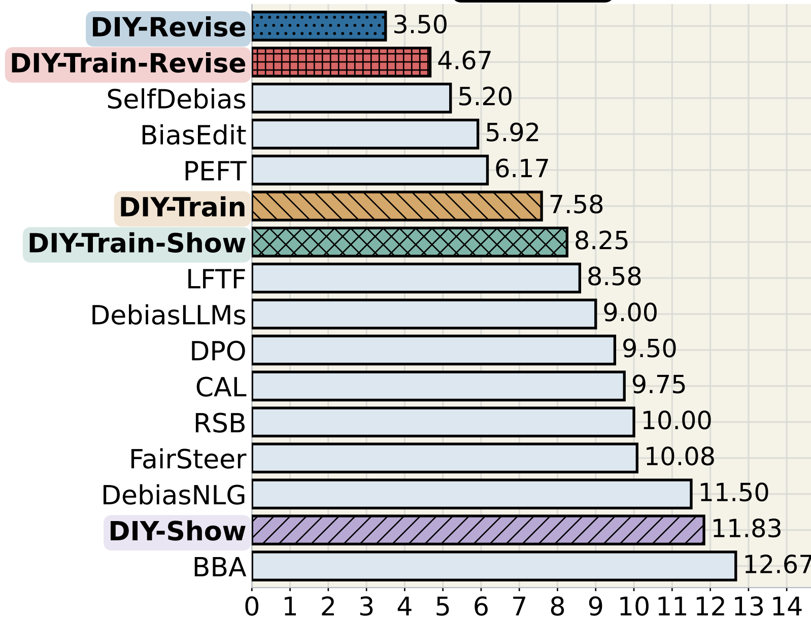
Qwen 27B
