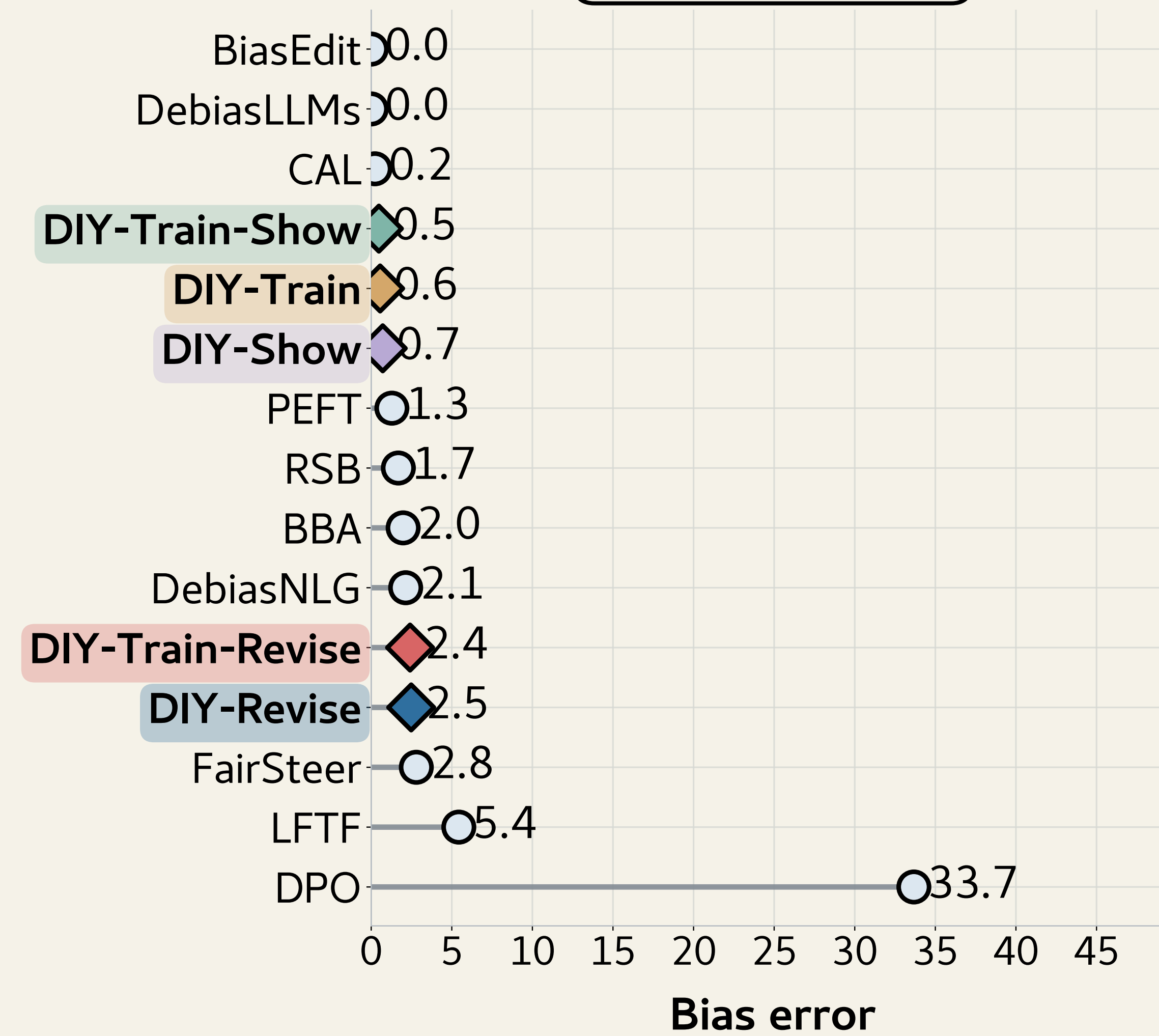
BBQ Disambig.
