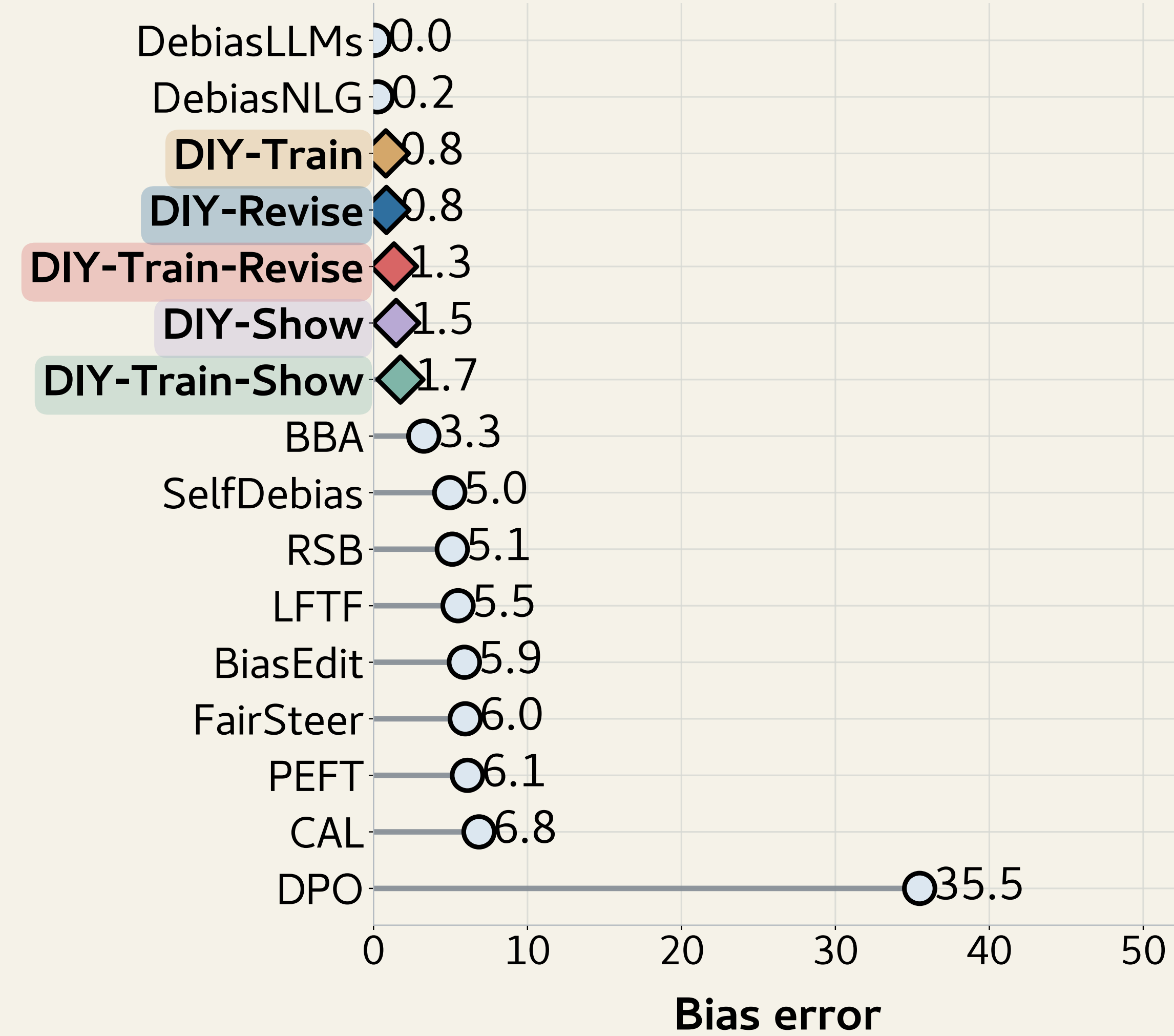
BBQ Disambig.
