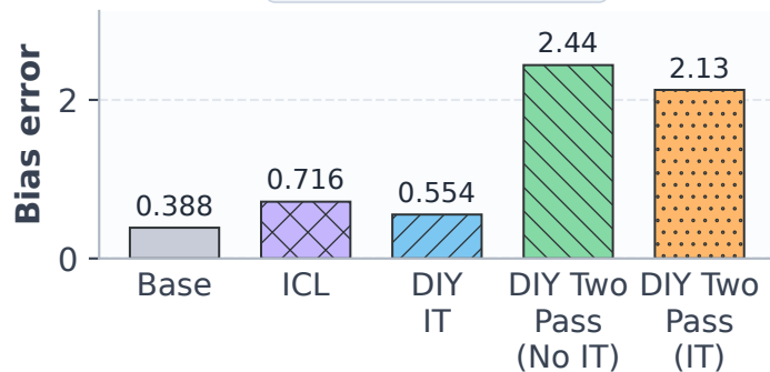
BBQ Disambig.
