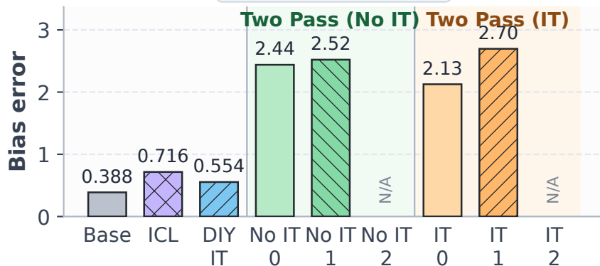
BBQ Disambig.
