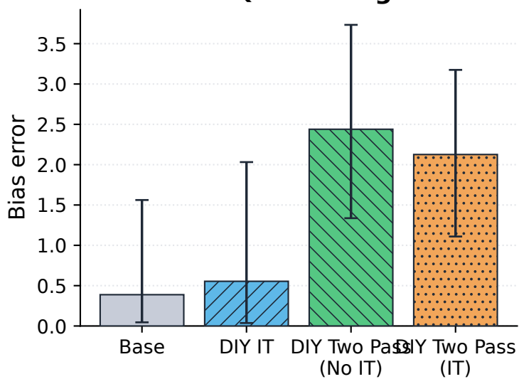
BBQ Disambig.
