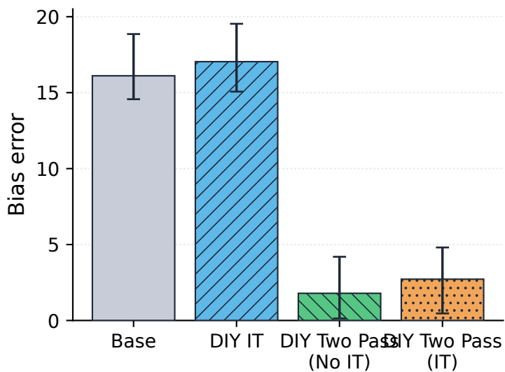
BBQ Disambig.
