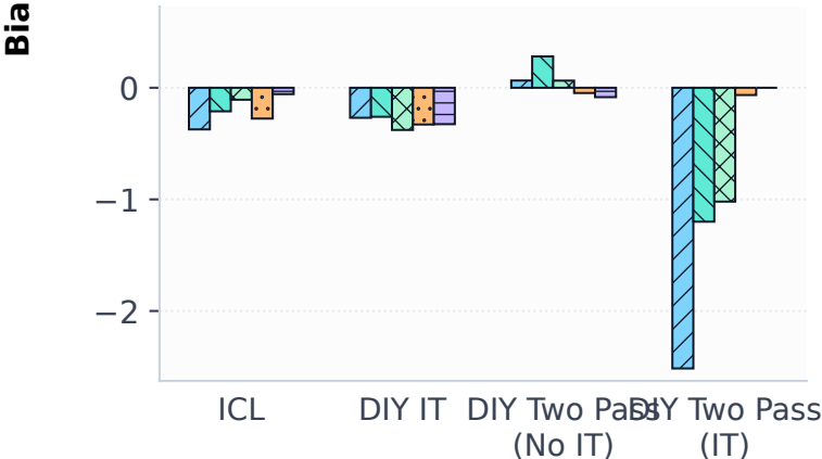
BBQ Disambig.
