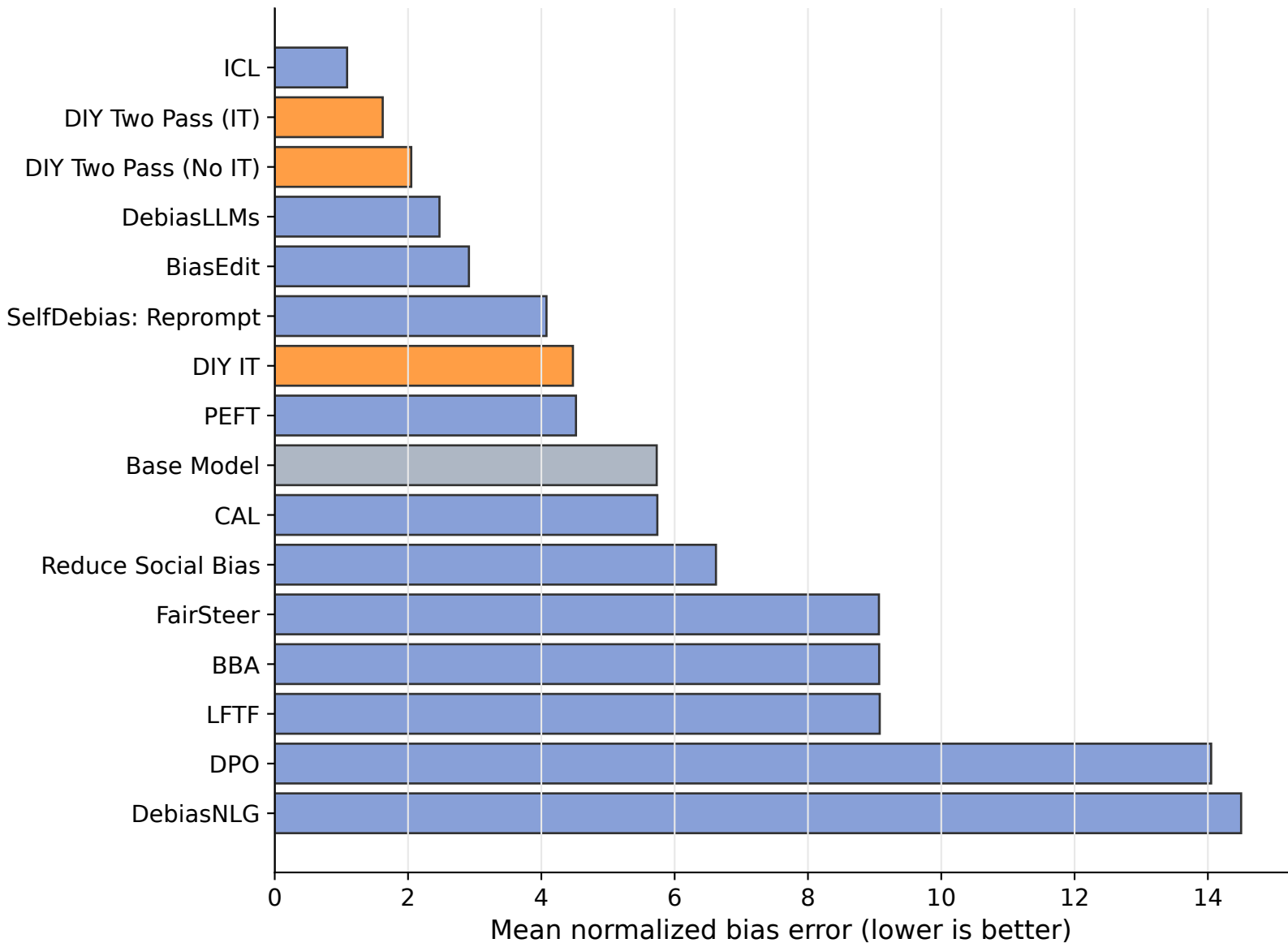
Mean Bias Error Across Benchmark Panels
