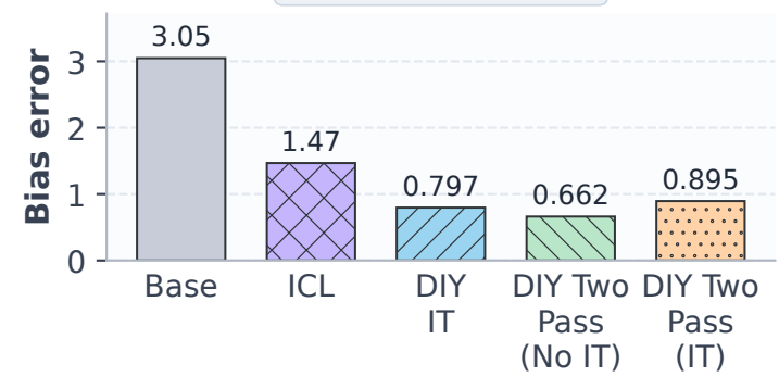
BBQ Disambig.
