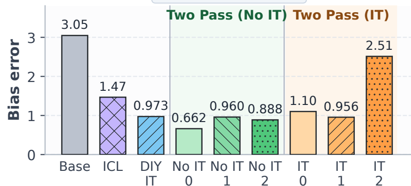
BBQ Disambig.
