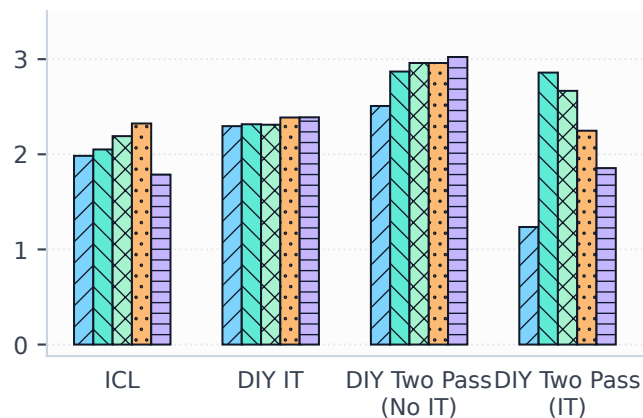
BBQ Disambig.
