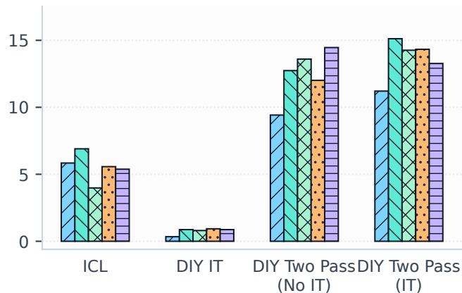
BBQ Disambig.
