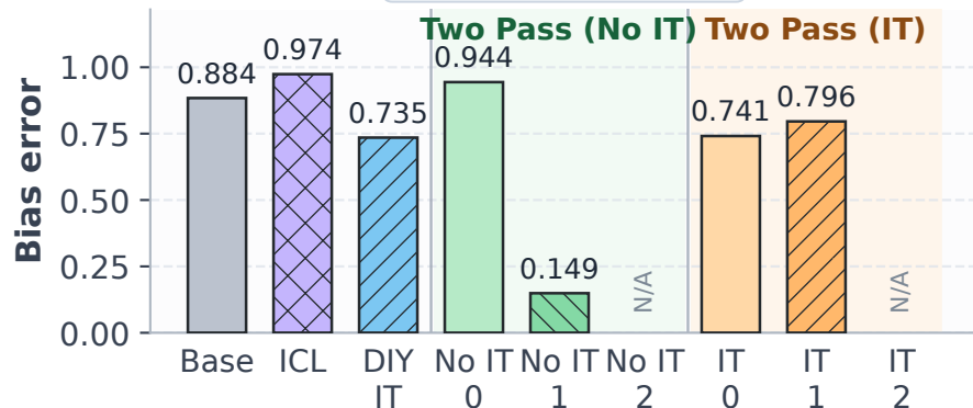
BBQ Disambig.
