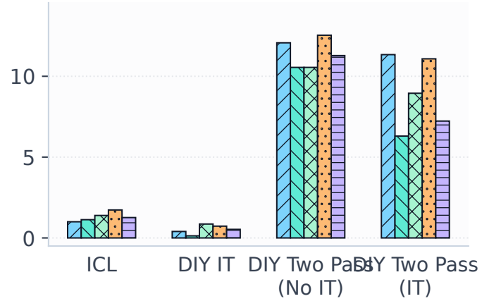
BBQ Disambig.
