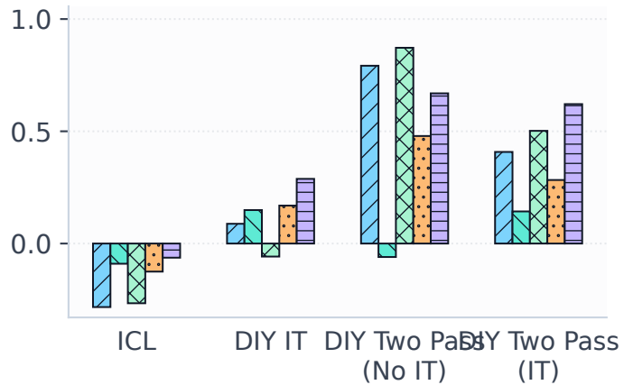
BBQ Disambig.
