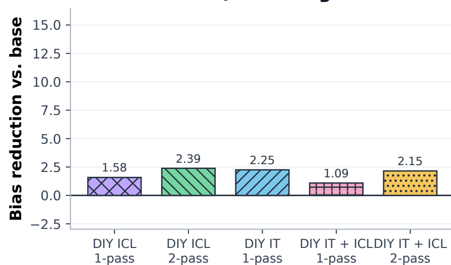
BBQ Disambig.
