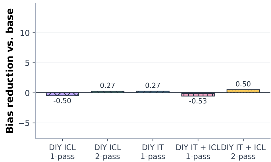
BBQ Disambig.
