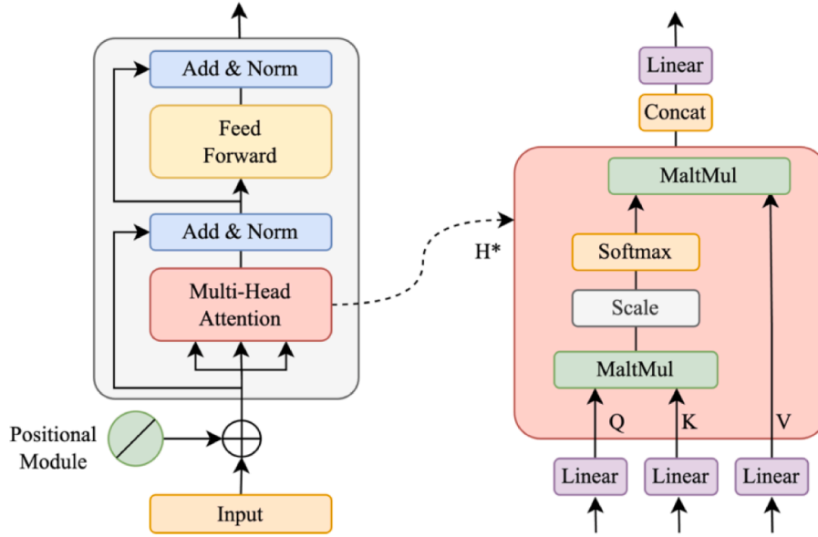
Fig. 4. Architecture of the Transformer sub-module.
