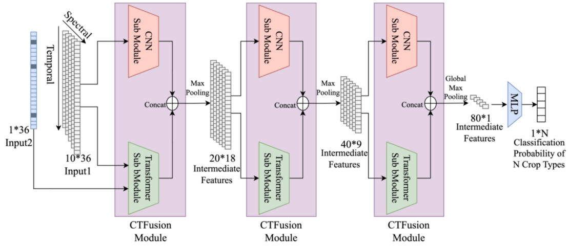
Fig. 3. Architecture of the MCTNet with three stages.
