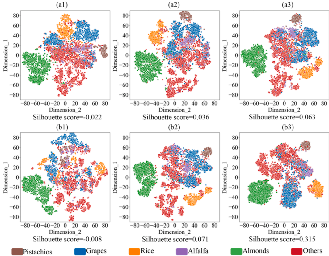
Fig. 14. The extracted feature distributions of (a) CNN sub-module, (b) Transformer sub-module from (1) the first stage to (3) the last stage in California.
