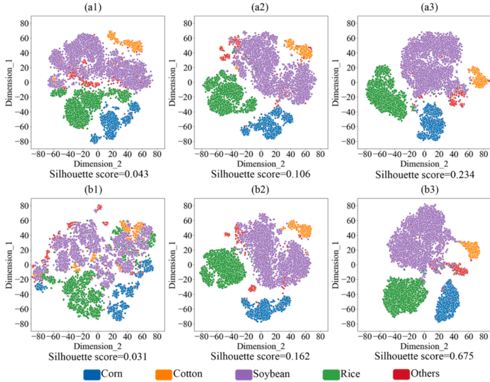
Fig. 13. The extracted feature distributions of (a) CNN sub-module, (b) Transformer sub-module from (1) the first stage to (3) the last stage in Arkansas.
