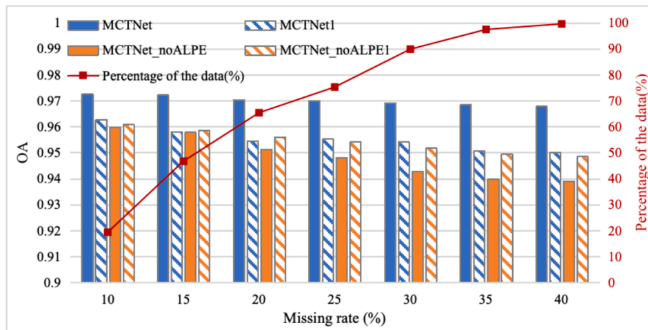
Fig. 15. The OA of the crop classification models using samples with different missing rates in Arkansas. (The red curve represents the percentage of the data that is less than a certain missing rate.). (For interpretation of the references to color in this figure legend, the reader is referred to the web version of this article.)
