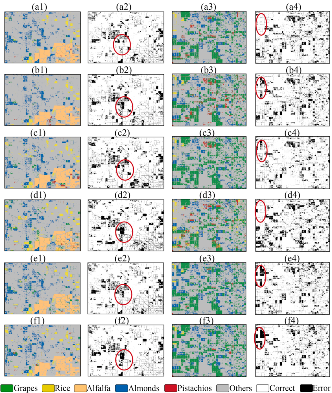
Fig. 10. Crop maps from (a) MCTNet, (b) GL-TAE, (c) LTAE, (d) ResNet, (e) Transformer, (f) RF in mapping area 1 (1) and mapping area 2 (3) in California. (2) and (4) represent the residual maps in mapping area 1 and mapping area 2, respectively.
