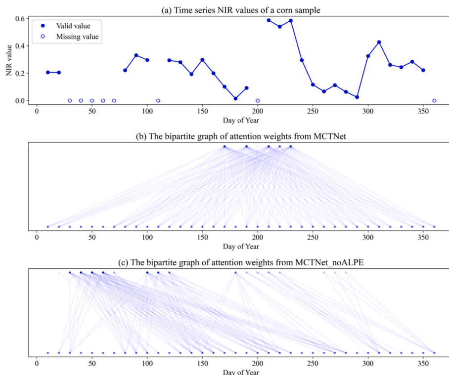
Fig. 17. Visual illustration of the attention weights from the MCTNet and MCTNet_noALPE.
