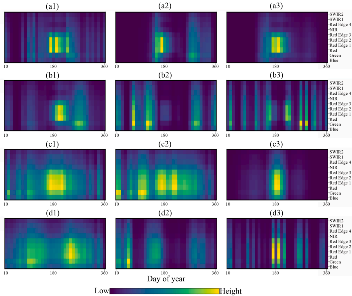
Fig. 12. Grad-CAM visualization results for (a) corn in Arkansas by CNN sub-module, (b) corn in Arkansas by Transformer sub-module, (c) grape in California by CNN sub-module, (d) grape in California by Transformer sub-module. (1) to (3) represent the tree stages in MCTNet. Yellow color indicates high-weight features, while blue color means low-weight features. (For interpretation of the references to color in this figure legend, the reader is referred to the web version of this article.)
