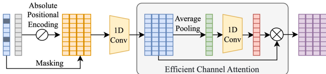
Fig. 5. Attention-based learnable positional encoding module.
