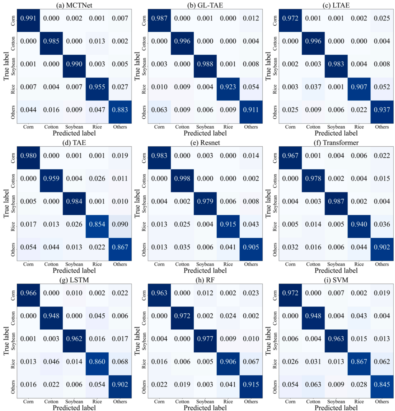
Fig. 7. Confusion matrices of different models in Arkansas.
