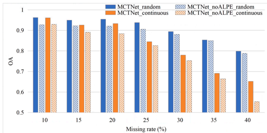
Fig. 16. Performance of the crop classification models using corn samples with different missing rates during the growing season ("random" denotes random missing data, "continuous" denotes continuous missing data).
