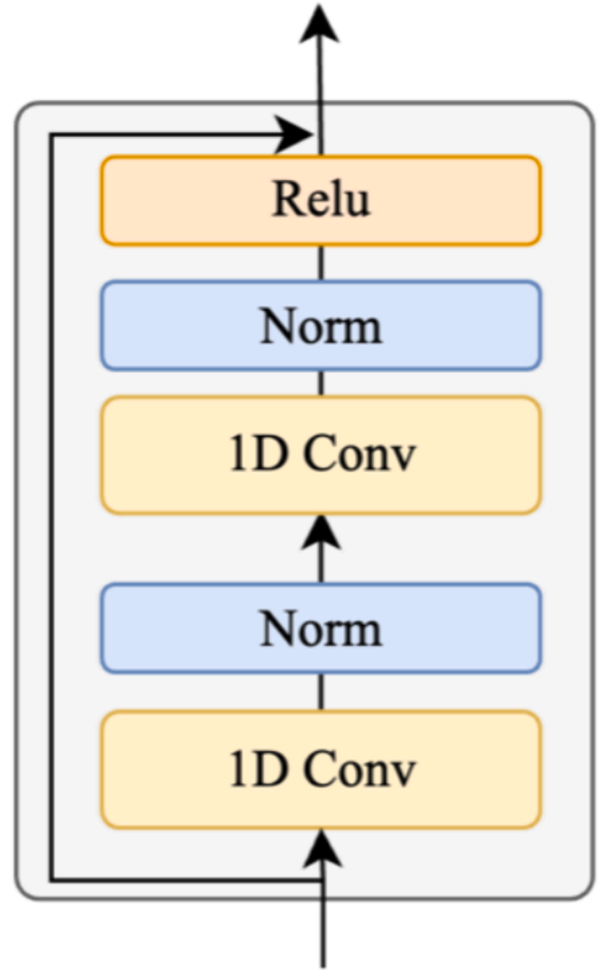
Fig. 6. Architecture of the CNN sub-module.
