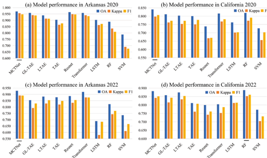
Fig. 11. Cross-temporal performance of different models (“_” represents the best model).
