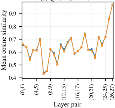
(a) Qwen2.5-VL-7B
