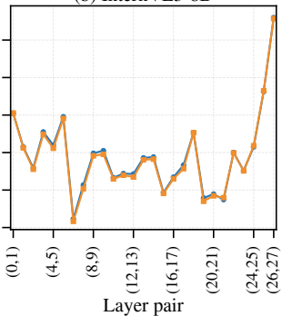
(b) InternVL3-8B
