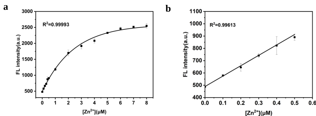
Fig. 2. a) Fluorescent response of the probe (1 \mu\text{M} ) to \text{Zn}^{2+} (0–8 \mu\text{M} ); b) Linear relationship between fluorescence intensity and \text{Zn}^{2+} concentration (0–0.5 \mu\text{M} ).
