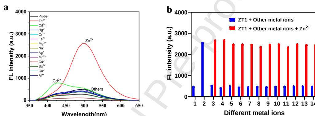
Fig. 1. a) Fluorescent response of ZT1 to various metal ions; b) Fluorescent selectivity of ZT1 with Zn^{2+} in the presence of various metal ions, including: 1- ZT1 , 2- Zn^{2+} , 3- Cd^{2+} , 4- Hg^{2+} , 5- Cr^{3+} , 6- Fe^{2+} , 7- Mg^{2+} , 8- Na^+ , 9- Ag^+ , 10- Mn^{2+} , 11- Co^{2+} , 12- Ba^{2+} , 13- Ca^{2+} , 14- Al^{3+} .
