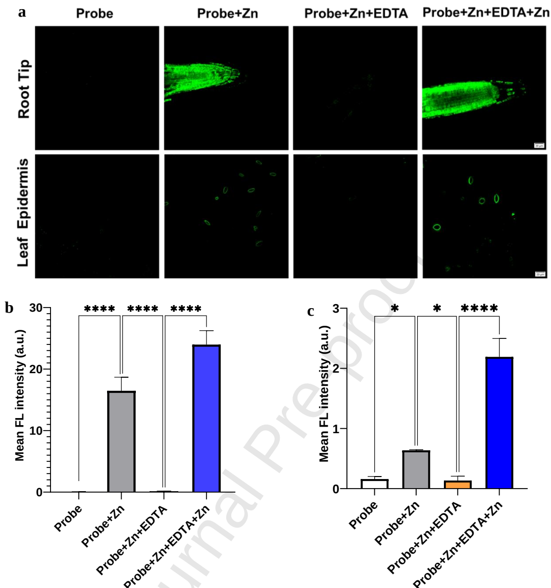
Fig. 6. a) Imaging of the probe (10 \mu M) in Arabidopsis root tips and leaves (Simple numbers n=3 , scale bar = 20 \mu m) in cyclic experiments; b) Average fluorescence intensity of root tips; c) Average fluorescence intensity of leaves.
