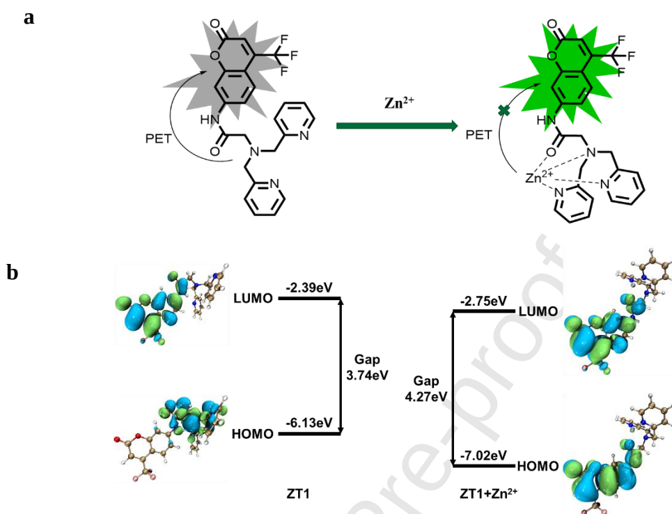
Fig. 3. a) The possible mechanism of the ZT1 ; b) HOMO and LUMO energy levels and the molecular orbital plots of ZT1 and ZT1-Zn 2+ . The structures of ZT1 and ZT1-Zn 2+ are obtained by conformational search using xtb 6.7.1 [42], Molclus 1.12 [43], ORCA 6.0.0 [44], and the plot was drawn using Multiwfn [45][46] and VMD 1.9.3 [47].
