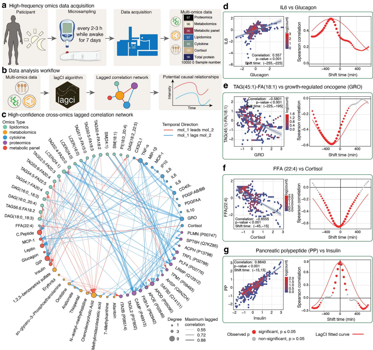
Figure 4 Inference of causal molecular relationships from high-frequency human multi-omics data. (a) High-frequency microsampling and multi-omics profiling of blood samples collected from one participant over 7 days. (b) Data analysis workflow. (c) High-confidence cross-omics lagged correlation network inferred by lagCI. Displayed edges were retained using stringent filtering criteria: quality score > 0.95, absolute maximum lagged correlation > 0.55, and Bonferroni-adjusted P < .001 . Up to the top 20 bridge nodes from each omics type were selected based on cross-omics degree. Node color indicates omics type, node size indicates degree, edge color indicates inferred temporal direction, and edge width represents the maximum lagged correlation estimated by lagCI. (d–g) Representative temporal relationships identified by lagCI. Observed lagged correlations are distinguished according to statistical significance ( P \leq .05 or P > .05 ), point size represents -\log_{10}(p \text{ value}) , and the curve shows the lagCI-fitted correlation profile.
