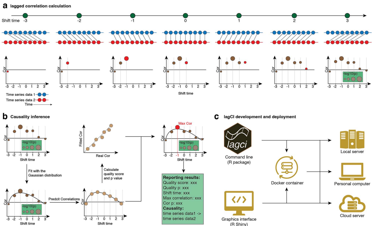
Figure 1 Overview of the lagCI algorithm for causal inference between time series. (a) Lagged correlation analysis. (b) Quality control and temporal causal relationship inference. (c) Software implementation and deployment.
