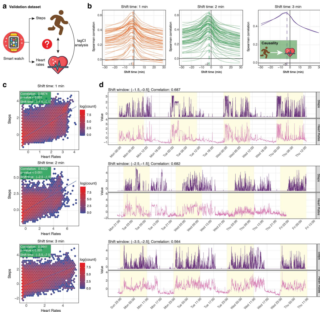
Figure 3 Validation of lagCI using step count and heart rate data from wearable smartwatches. (a) Schematic overview of the validation dataset. (b) Distribution of lagged correlation profiles across participants, stratified by peak correlation occurring at 1-min, 2-min, or 3-min lag. (c) Hexbin scatterplots of steps versus heart rate for one representative participant from each group. (d) Time series plots of step counts and heart rate for the same three representative participants.
