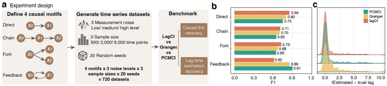
Figure 2 Simulation benchmark of lagCI with known causal ground truth. (a) Simulation experiment design. (b) Causal-link recovery across four causal motifs. (c) Lag-time estimation accuracy on recovered edges.
