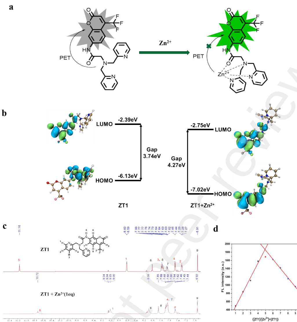
Fig. 3. a) The possible mechanism of the ZT1 ; b) HOMO and LUMO energy levels and the molecular orbital plots of ZT1 and ZT1-Zn 2+ . The structures of ZT1 and ZT1-Zn 2+ are obtained by conformational search using xtb 6.7.1[33], Molclus 1.12[34], ORCA 6.0.0[35], and the plot was drawn using Multiwfn [36][37] and VMD 1.9.3[38]; c) 1 H NMR spectra of ZT1 in the presence of Zn 2+ in DMSO-d 6 ; d) J-job curve of ZT1 .
