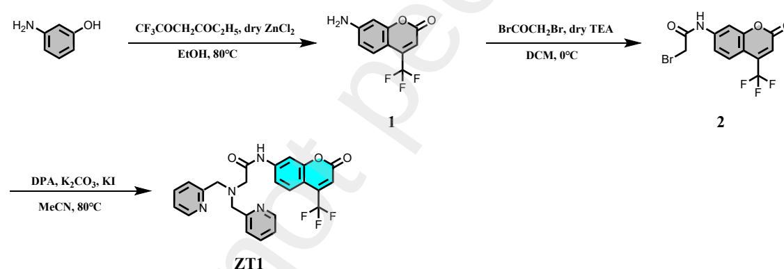
Scheme 1. The synthetic route of probe ZT1 .
