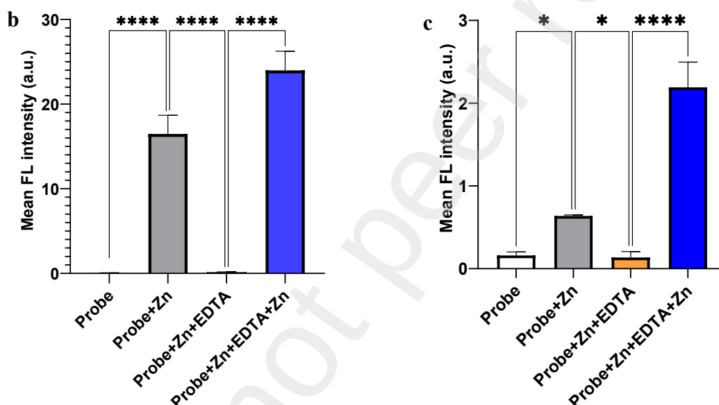
Fig. 6. a) Imaging of the probe (10 \mu M) in Arabidopsis root tips and leaves (Simple numbers n=3, scale bar = 20 \mu m) in cyclic experiments; b) Average fluorescence intensity of root tips; c) Average fluorescence intensity of leaves.
