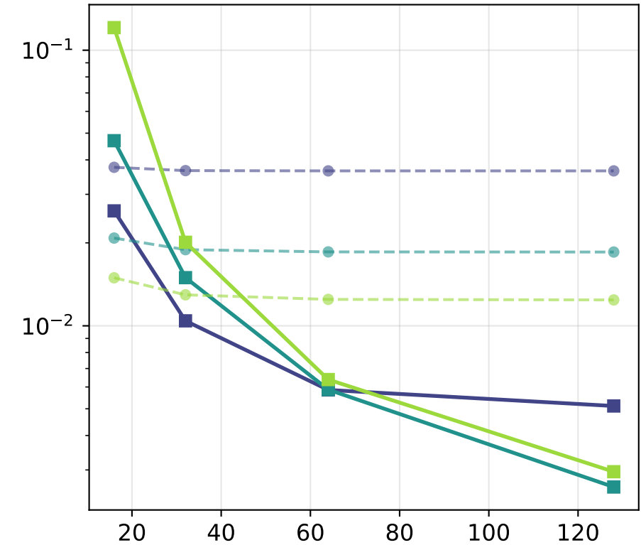
Quarter-fill U=4 (metallic)
