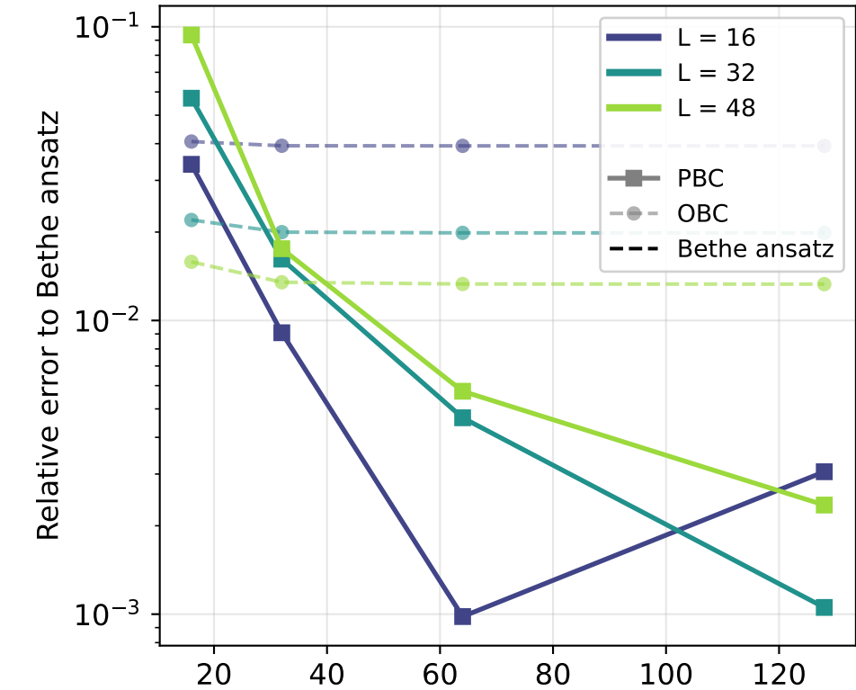
Half-fill U=4 (gapped)
