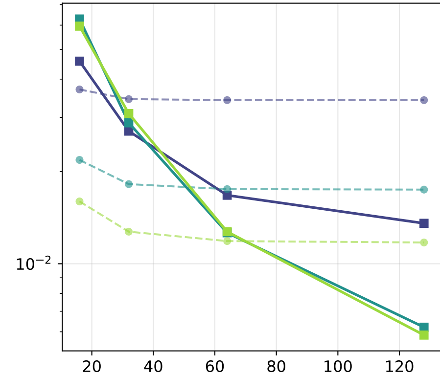
Half-fill U=0 (free fermion)
