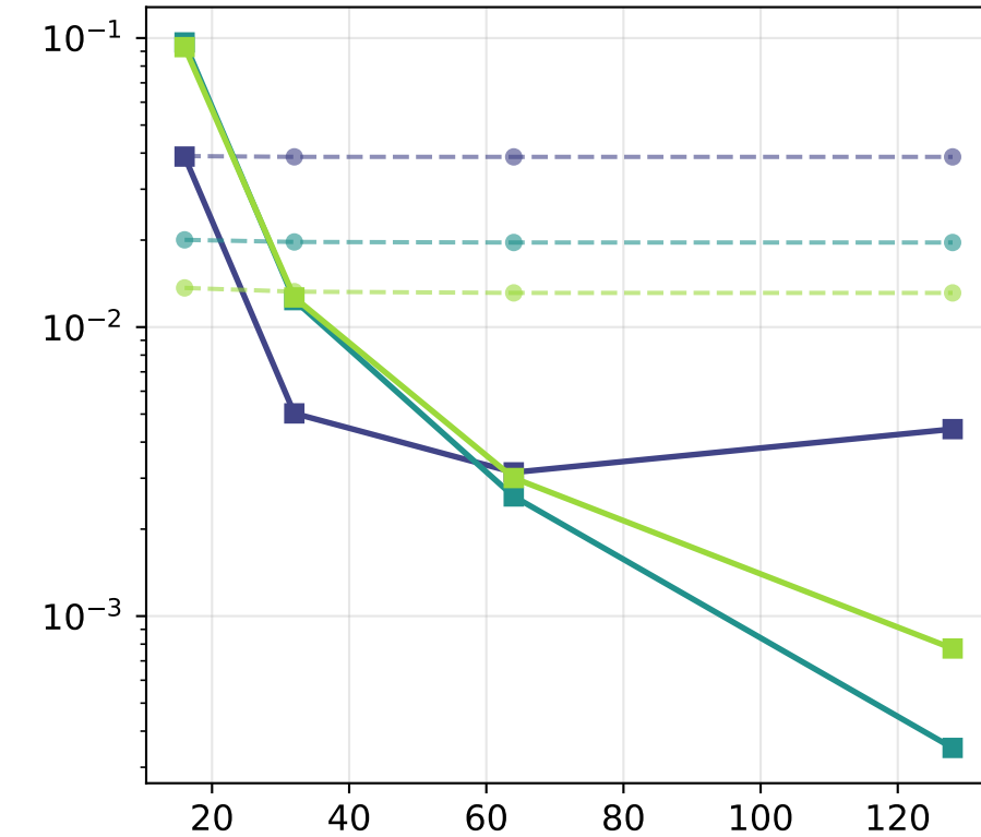
Half-fill U=8 (strongly gapped)
