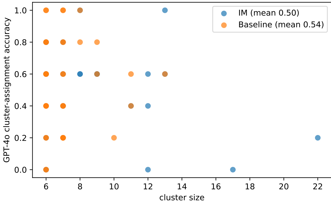
Fig 3: interaction-metric feature clusters (ckubmeg1, \lambda=1000 )
